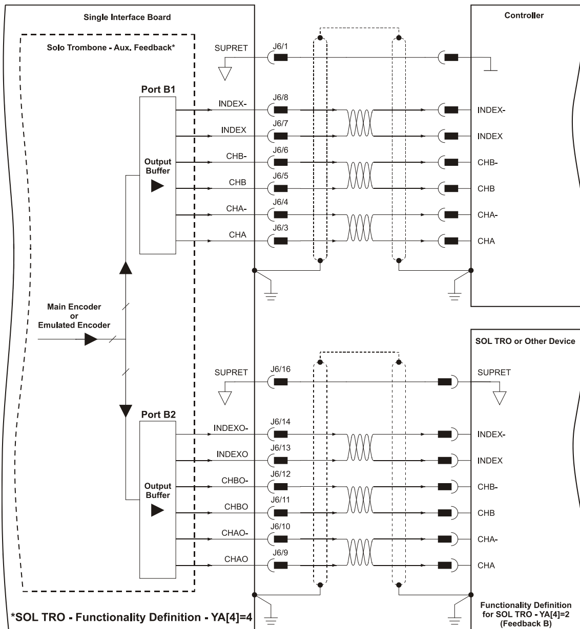
Figure 20: Emulated Encoder Direct Output – Acceptable Connection Diagram
